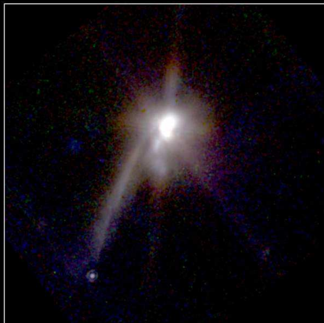
TMR-1C • Protoplanet in Taurus HST • NICMOS PRC98-19 • ST ScI OPO • May 28, 1998 S. Terebey (Extrasolar Research Corp.) and NASA
